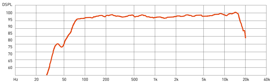
SPL vs Freq
